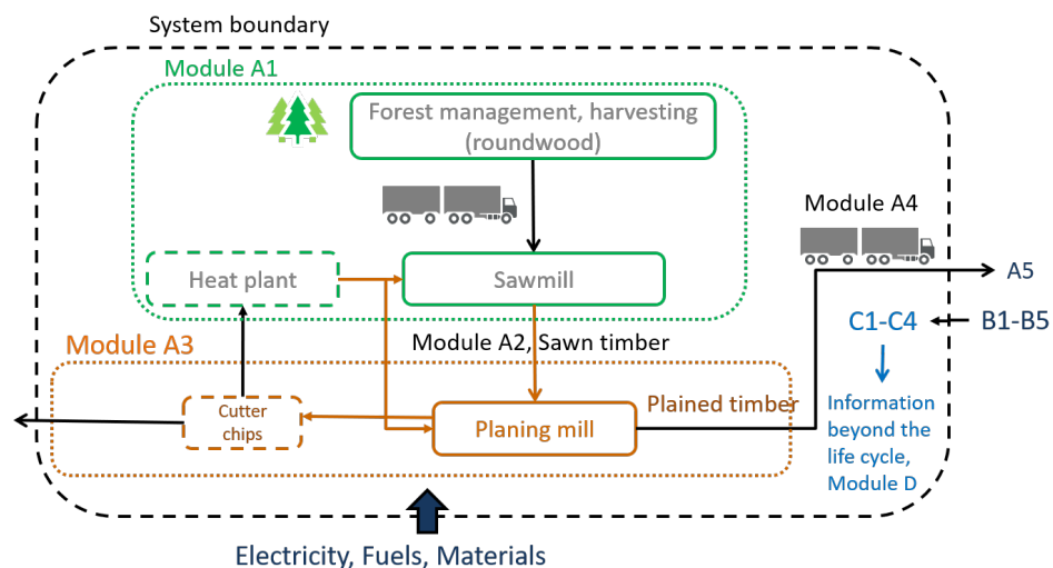
Figure 1. System boundary of planed timber EPD. The key inventoried flows.
